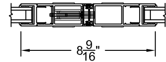
1" SIGHTLINE EXTENDER
