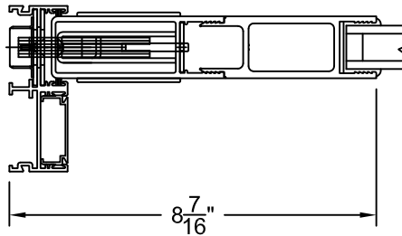
3.5" SIGHTLINE EXTENDER
