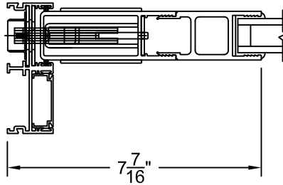
2.5" SIGHTLINE EXTENDER
