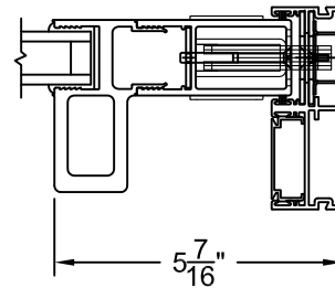
HP1 ADAPTER
