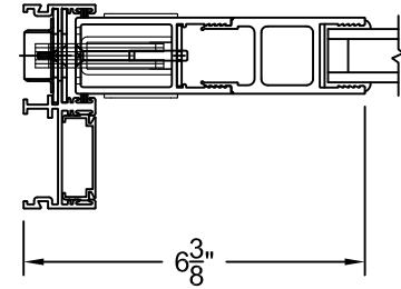
2.5" SIGHTLINE EXTENDER
