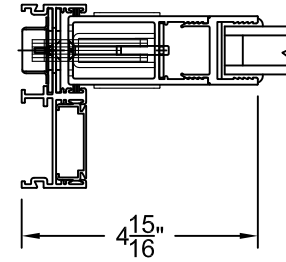
1" SIGHTLINE EXTENDER
