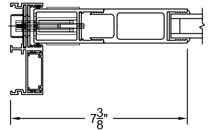
3.5" SIGHTLINE EXTENDER
