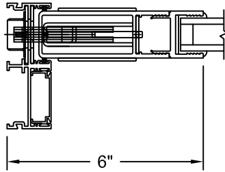
1" SIGHTLINE EXTENDER
