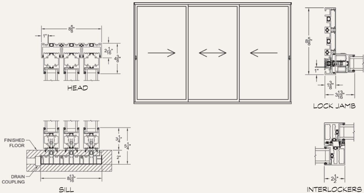
ELEVATION VIEW: XXX CONFIGURATION
